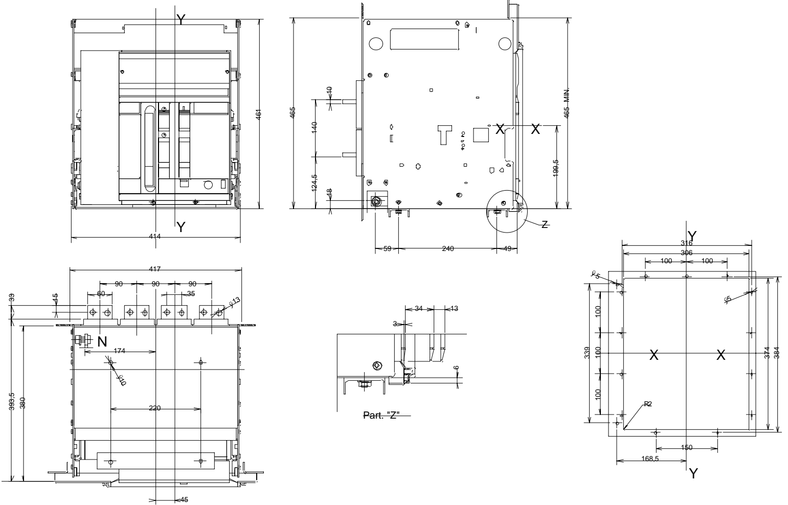
E1 4 POLE DRAW-OUT VERSION HORIZONTAL REAR TERMINALS
