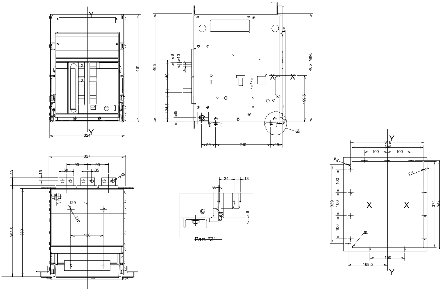
E2 3 POLE DRAW-OUT VERSION HORIZONTAL REAR TERMINALS
