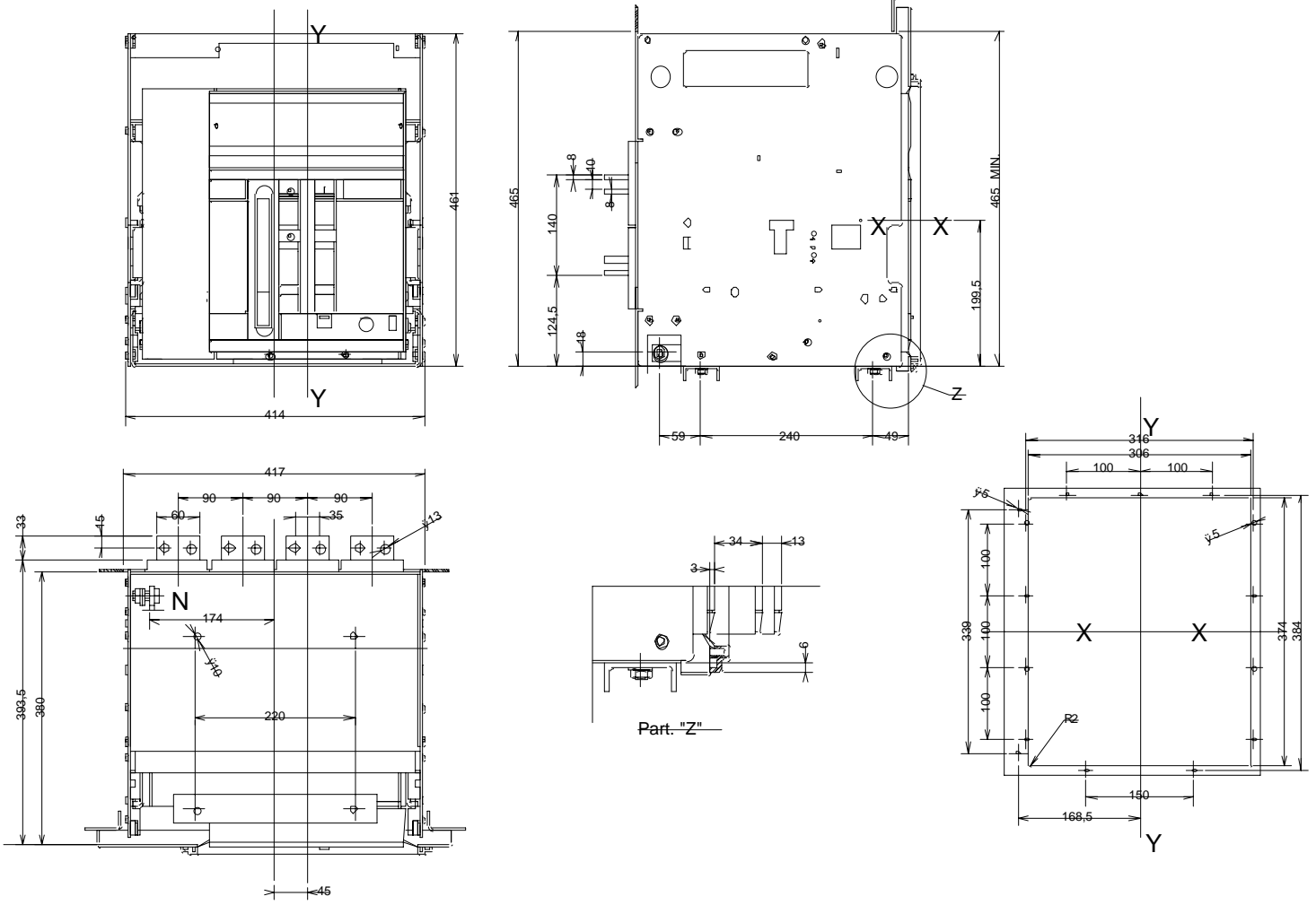
E2 4 POLE DRAW-OUT VERSION HORIZONTAL REAR TERMINALS
