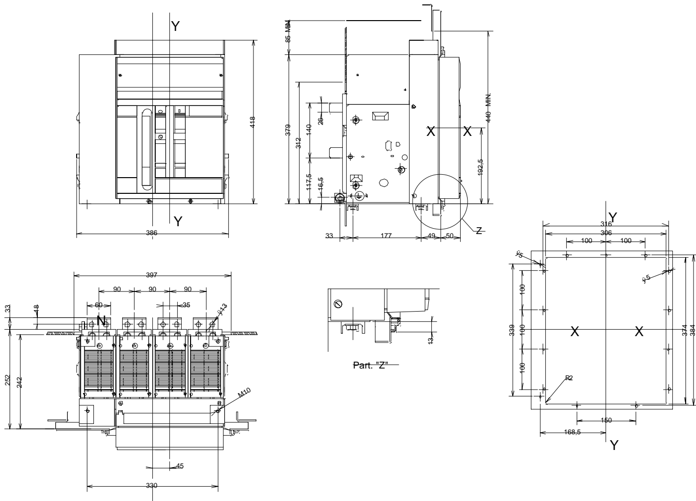
E2 4 POLE FIXED VERSION HORIZONTAL REAR TERMINALS
