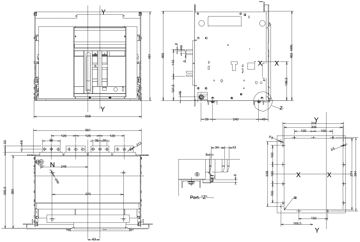
E3 4 POLE DRAW-OUT VERSION HORIZONTAL REAR TERMINALS All dimensions in mm
