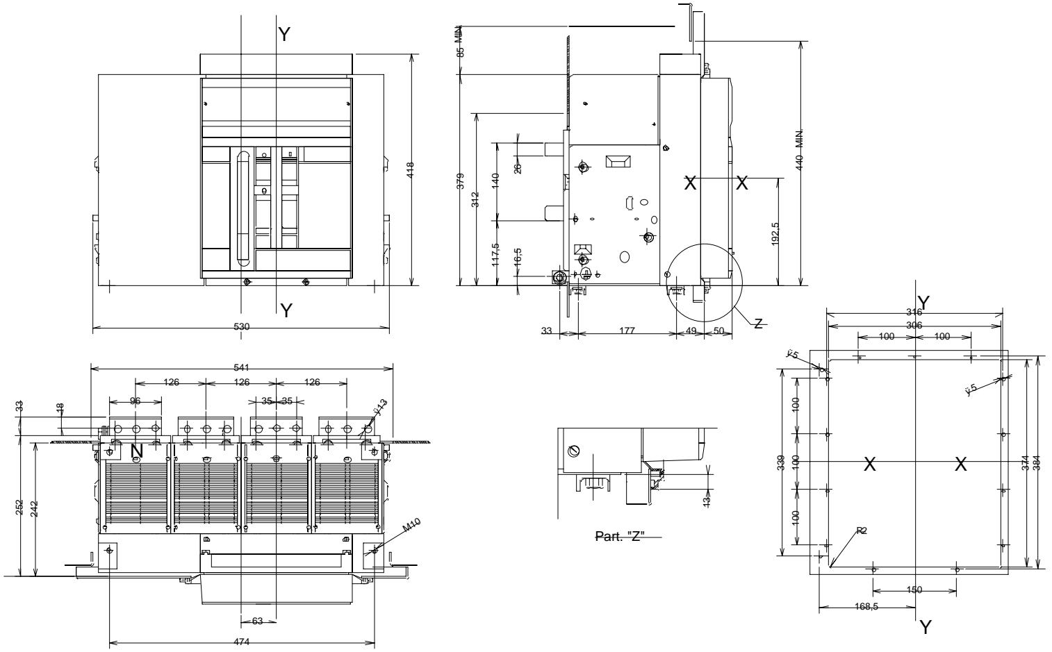
E3 4 POLE FIXED VERSION HORIZONTAL REAR TERMINALS
