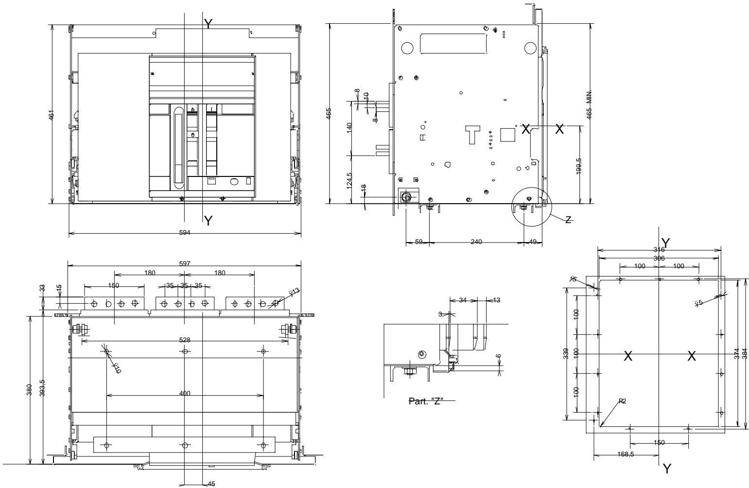
E4 3 POLE DRAW-OUT VERSION HORIZONTAL REAR TERMINALS All dimensions in mm
