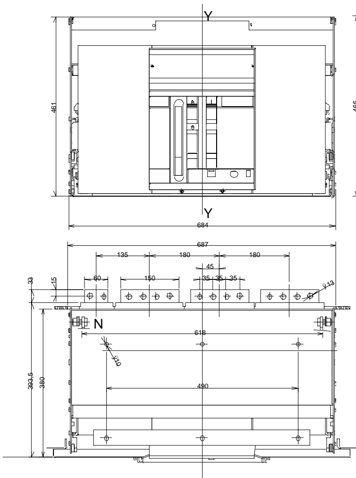
E4 4 POLE DRAW-OUT VERSION HORIZONTAL REAR TERMINALS All dimensions in mm
