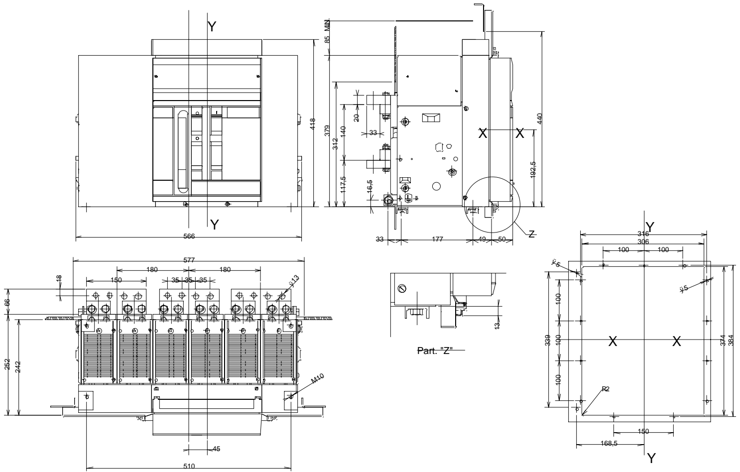
E44 POLE FIXED VERSION HORIZONTAL REAR TERMINALS All dimensions in mm
