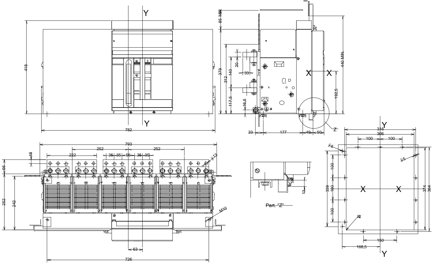
E6 3 POLE FIXED VERSION HORIZONTAL REAR TERMINALS All dimensions in mm
