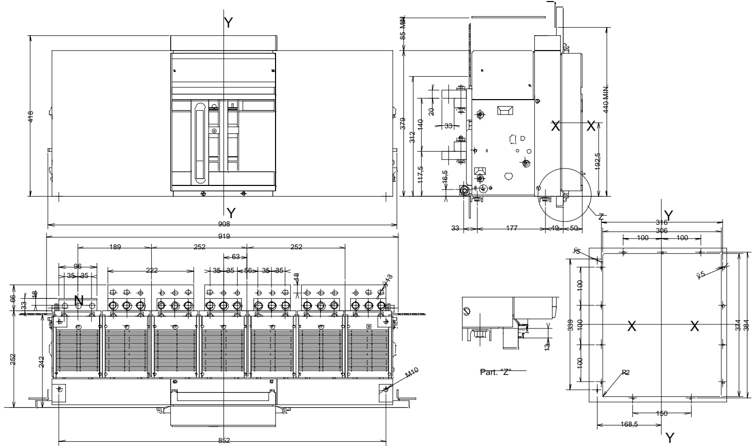
E6.4 POLE FIXED VERSION HORIZONTAL REAR TERMINALS All dimensions in mm
