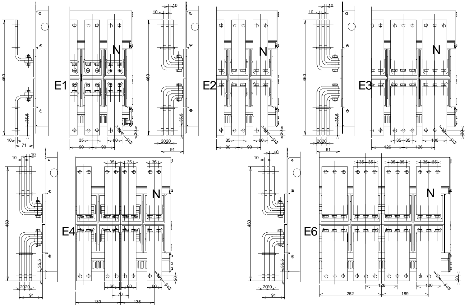
FRONT TERMINALS E1-E6 DRAW-OUT VERSION All dimensions in mm
