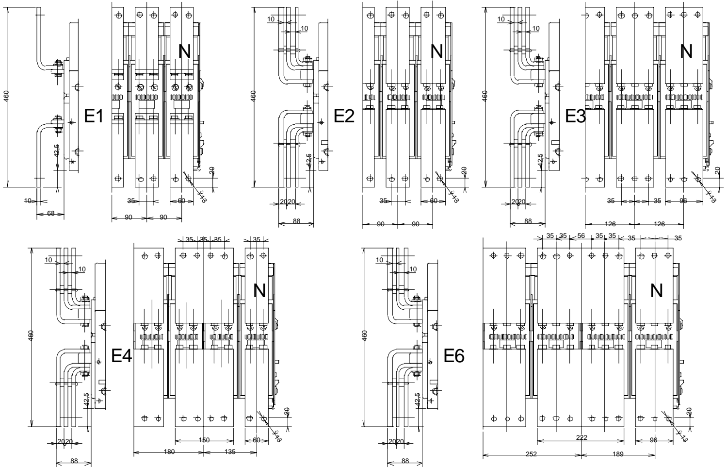
E1-E6 FRONT TERMINALS FIXED VERSION
