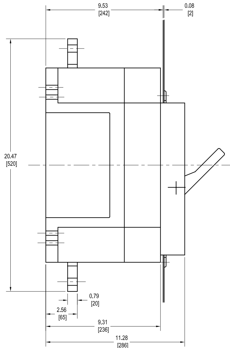
3 POLE LOW VOLTAGE M.C.C.B. M.C.S. SERIES "ISOMAX" FIXED VERSION FRONT TERMINALS
