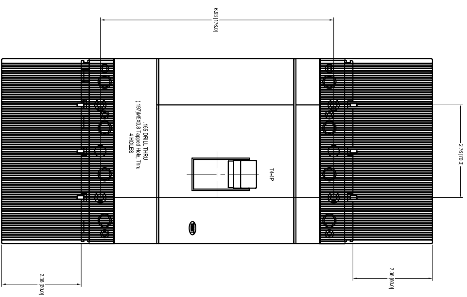
DRILL THRU
