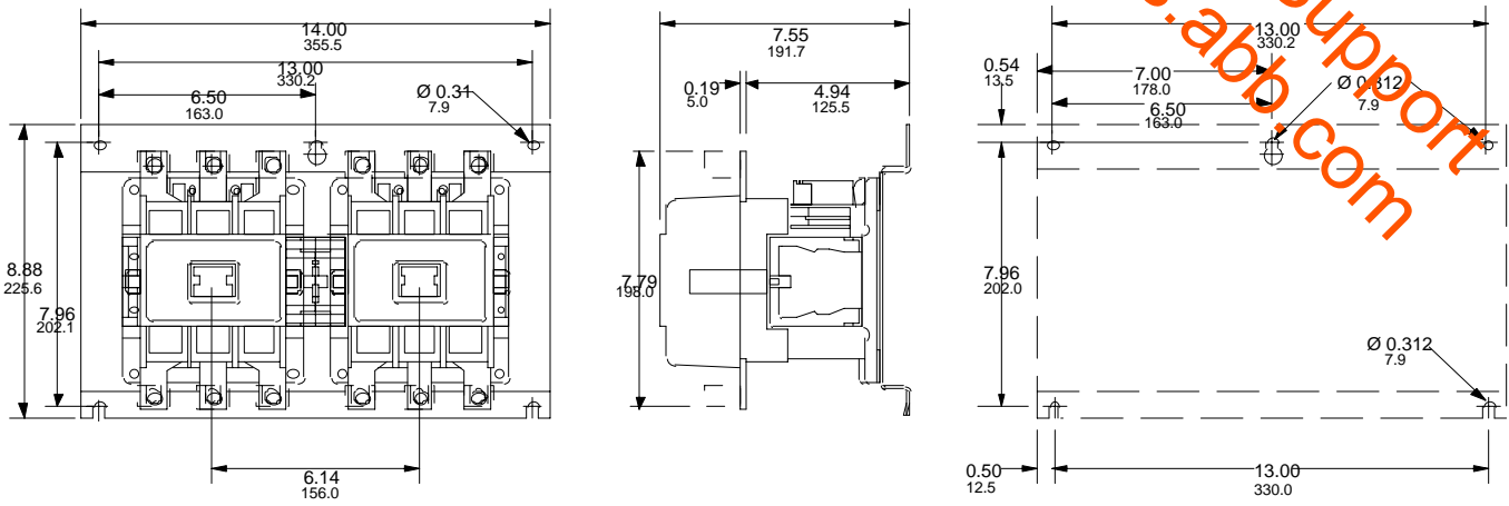
EH210M.I. Contactor W/EHTK210
