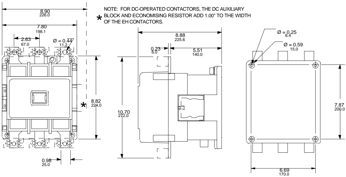
EH 450 Contactor
