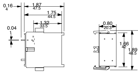
AUXILIARY SWITCH BLOCK CA 6-P
