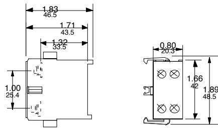
AUXILIARY SWITCH BLOCK CA 6
